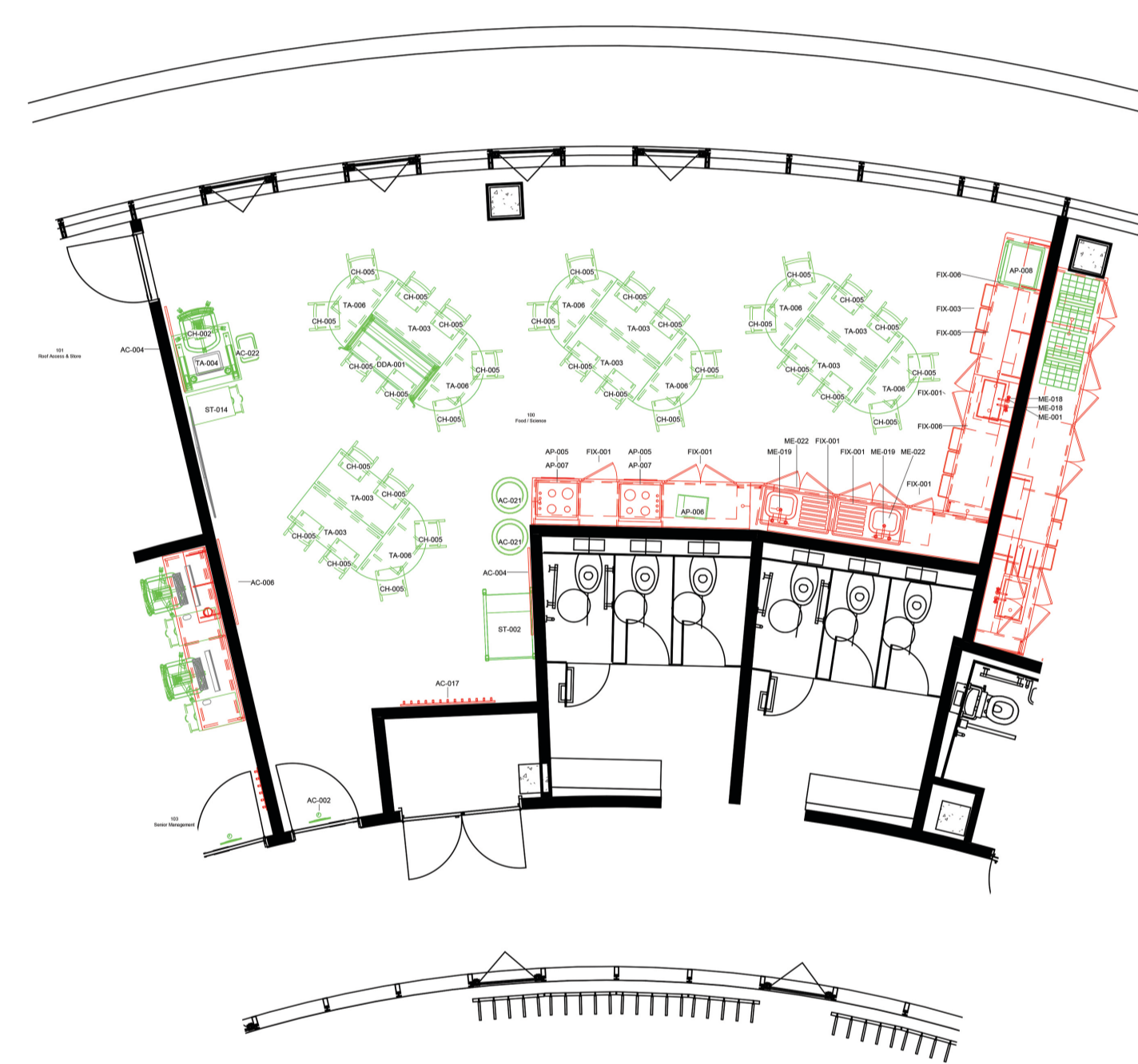
1 FF&E Room Plan - Food - Science 1:45
